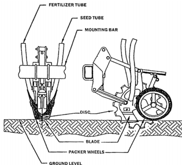
Fig. 2. Cross Slot assembly mounted on parallelogram drag arms (Baker et al., 1996).
